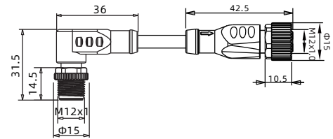
8Pins
