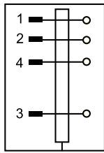
Male, Straight
