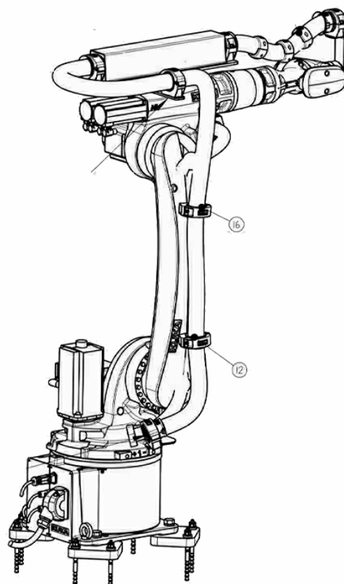
FA-KUKA-KR16-R1610-SW-1-6A
