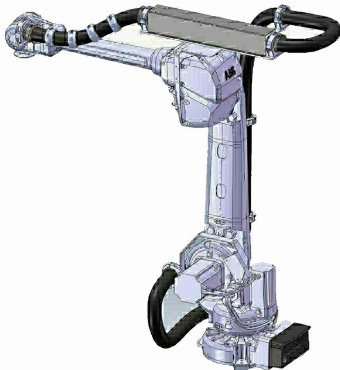
FA-ABB-IRB4600-SW-1-6A
