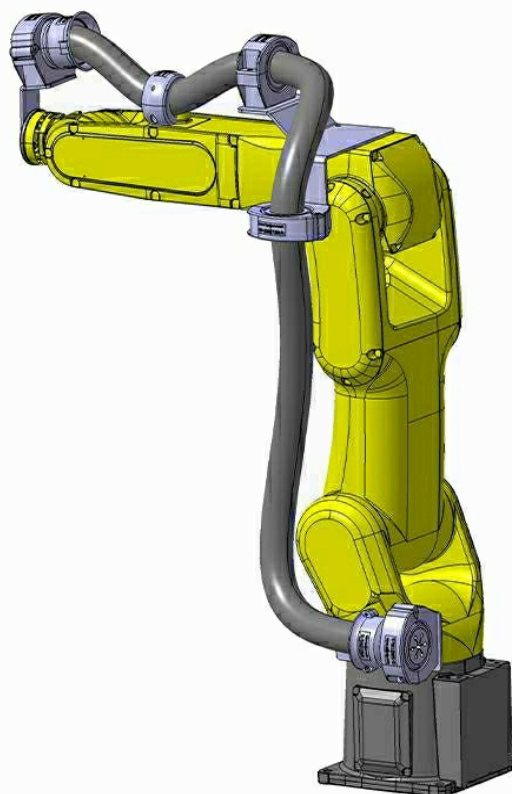
FA-FANUC-200iD7L-ARC-1-6A
